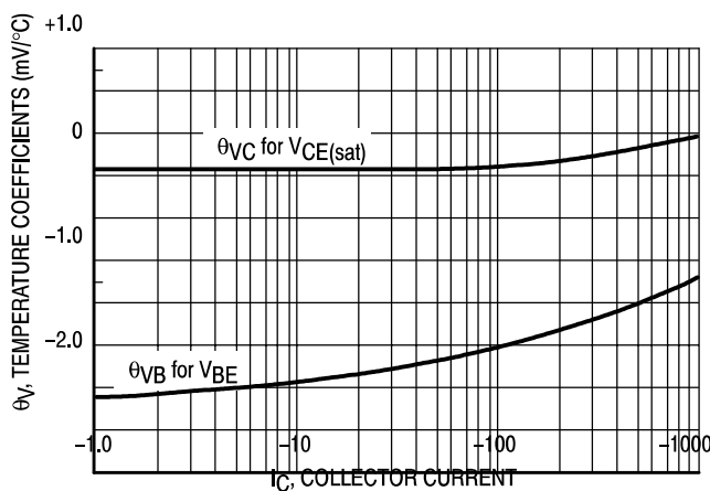
Figure 4. Temperature Coefficients
