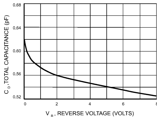
Figure 4. Capacitance
